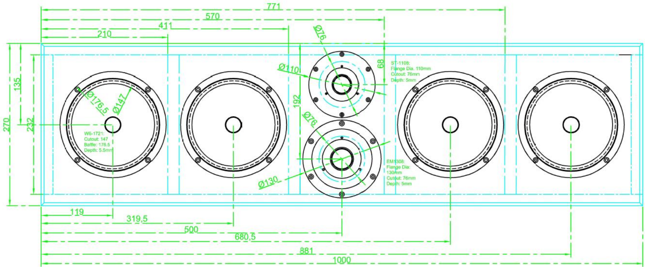
Centre Speaker Front View and Dimensions
